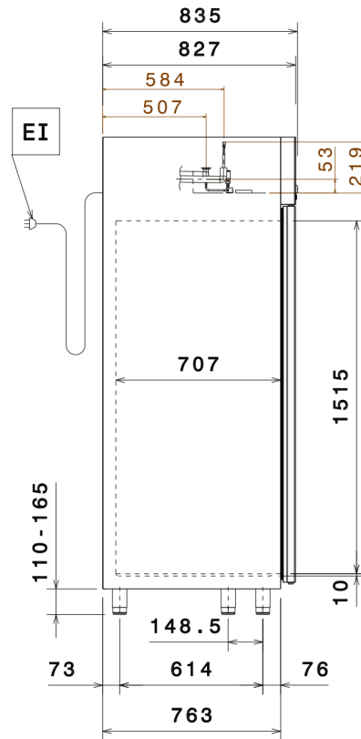
Side
